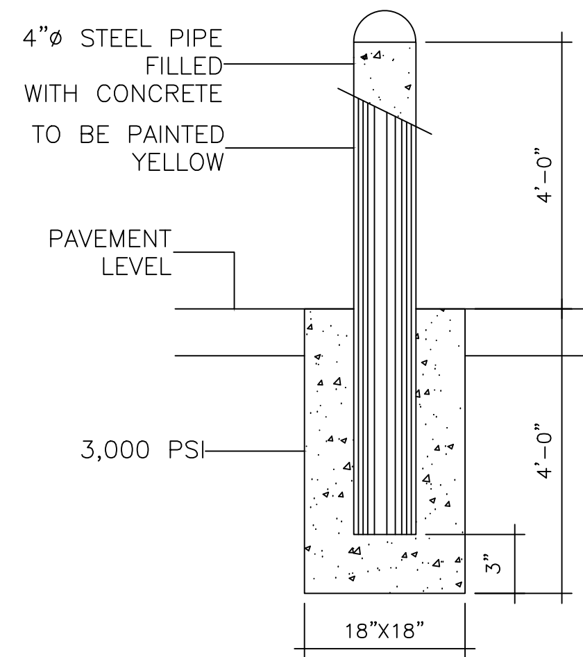
PROTECTION PIPE DETAIL
