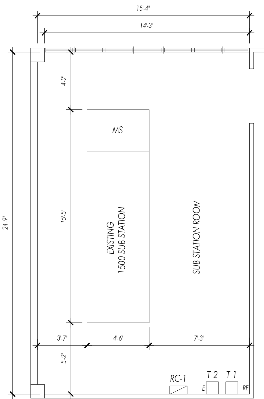
EXISTING SUBSTATION ROOM BLOW UP
