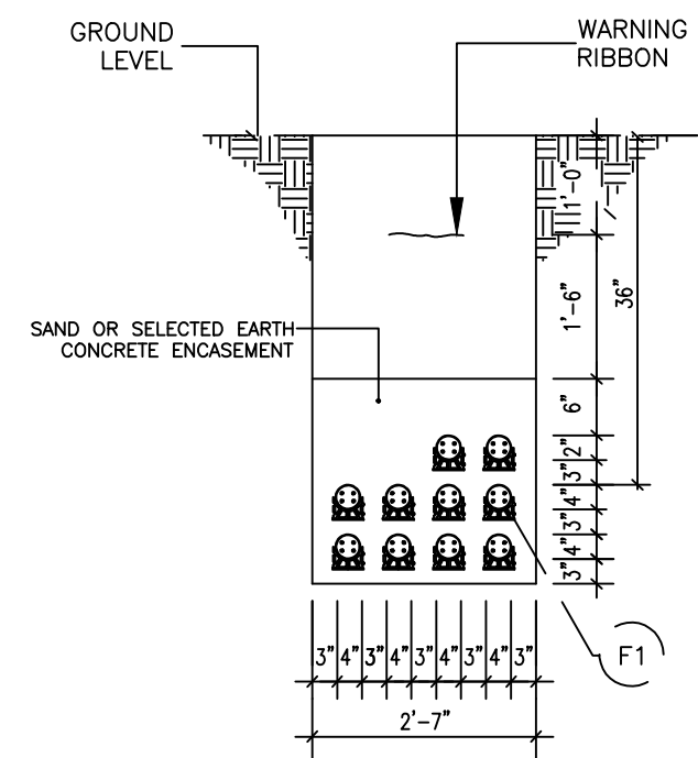
TRENCH DETAIL A-A
