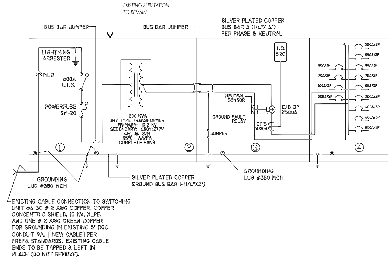
EXISTING ONE LINE DIAGRAM
